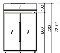
Integral front elevation
