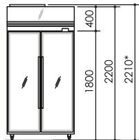
Integral front elevation
