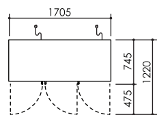
Integral top view
